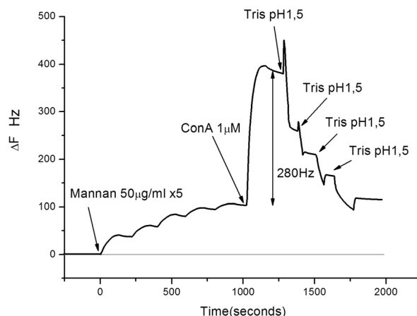
Fig. 1 Con A immobilization on mannan film on a ODT hydrophobic surface of a QCM electrode.
